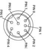
8-PIN DIN MALE MATING FACE
